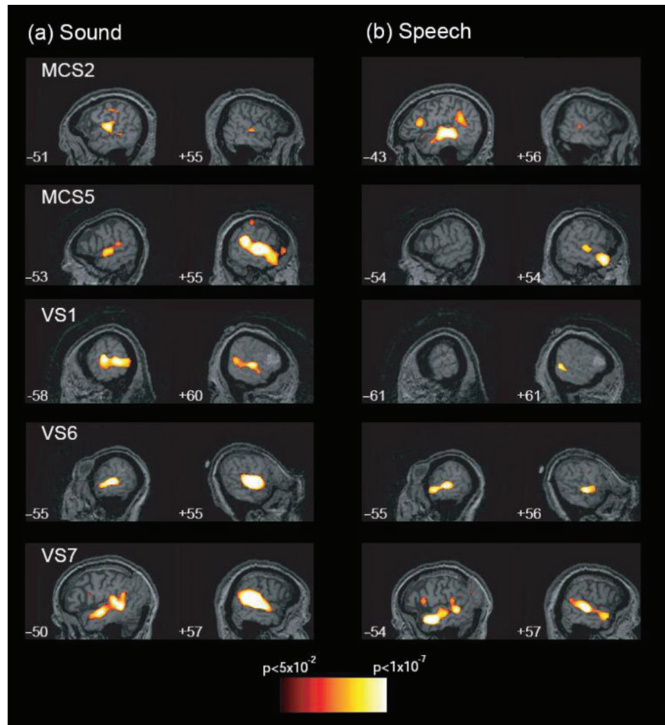
Fig. 4 Results for patients who met the diagnostic criteria for either the VS or the MCS, and who showed significant differences for all sound versus silence (A) and intelligible speech versus unintelligible noise (B). Activations are thresholded at P < 0.05 FDR corrected for multiple comparisons and shown on slices where the peak activation was observed.
