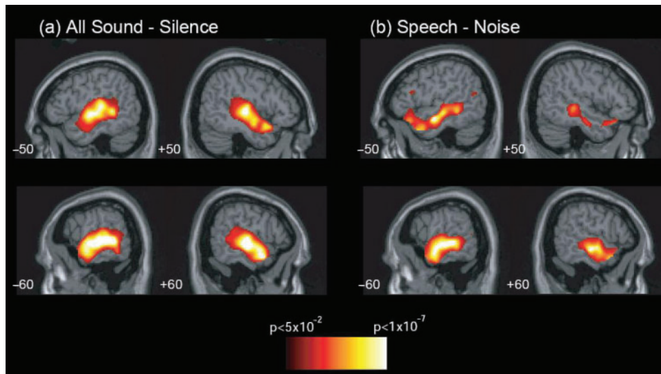
Fig. 1 Results from random effects group analyses of healthy volunteers (Data from Rodd et al. , 2005, Expt 2) for all sound versus silence (A) and intelligible speech versus unintelligible noise (B) . Activations are thresholded at P < 0.05 FDR corrected for multiple comparisons.
